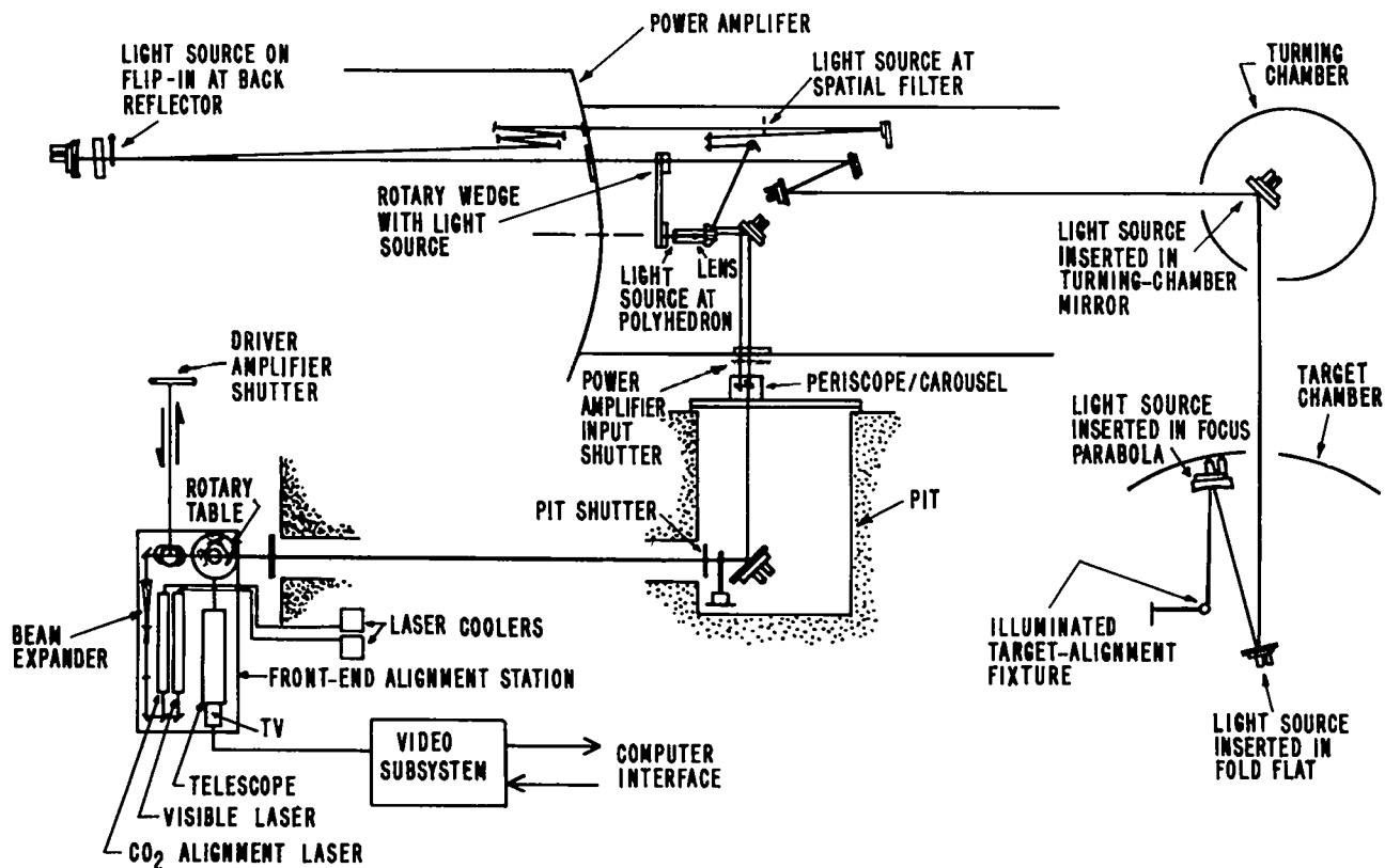
Fig. II-9. Antares automatic alignment schematic. The optical alignment path extends from the front-end room through the power amplifier and TVS onto the target position.
