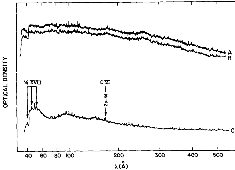
Fig. V-10. Microdensitometer scans of nickel Solacel targets: (a) through the center and (b) 300 \mu\text{m} from the center of a 5.2-kJ laser shot; (c) low-energy result at \sim 20 J.
