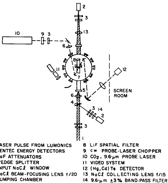
Fig. II-25. Experimental setup to investigate plasma formation.
