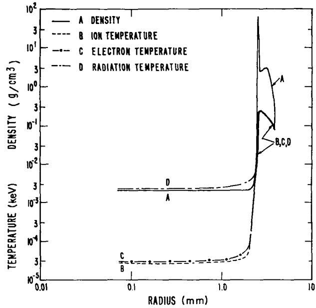
Fig. VIII-4. Temperature and density profiles of pellet at ion-beam turnoff show regional behavior of target.
