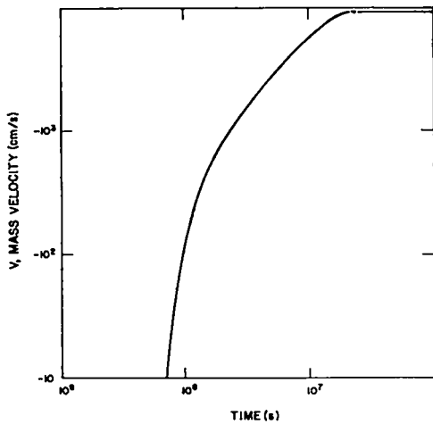
Fig. IX-6. The development of mass velocity associated with x-ray energy deposition ( S_0 = 5 \times 10^{17} erg/cm 3 ·s).
