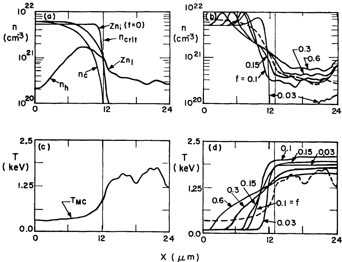
Fig. IV-7. Ablation calculated [(a),(c)] with Monte Carlo, and [(b),(d)] through flux-limited single-group diffusion, \cdots T_{mc} , -T_d . Diffusion critical fiducial is for f = 0.6 .
