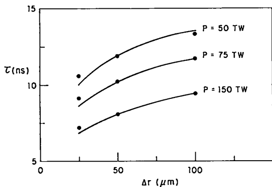
Fig. VIII-11. Collapse time vs shell thickness for 1-mm-radius targets.
