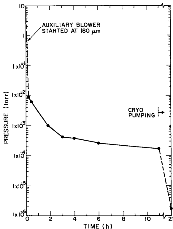
Fig. II-6. Electron-gun pumpdown time with cryogenic pump.
