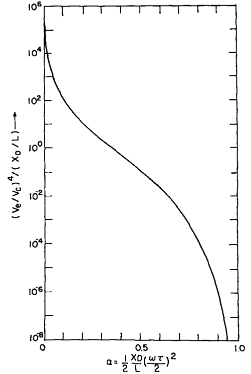
Fig. IV-2. Solution of Eq. (IV-25) of the text, (v_e/v_e)^4/(x_D/L) vs \alpha , provides approximate wave-breaking or convective saturation time given driver amplitude, background plasma temperature, and density scale length.
