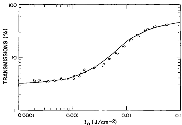
Fig. VII-7. Saturable absorption in 1.25 \times 10^{-3} molecules/cm 3 anthracene in n-hexane saturated with air. Theory (solid line), data set 1 (closed circles), and data set 2 (open circles).
