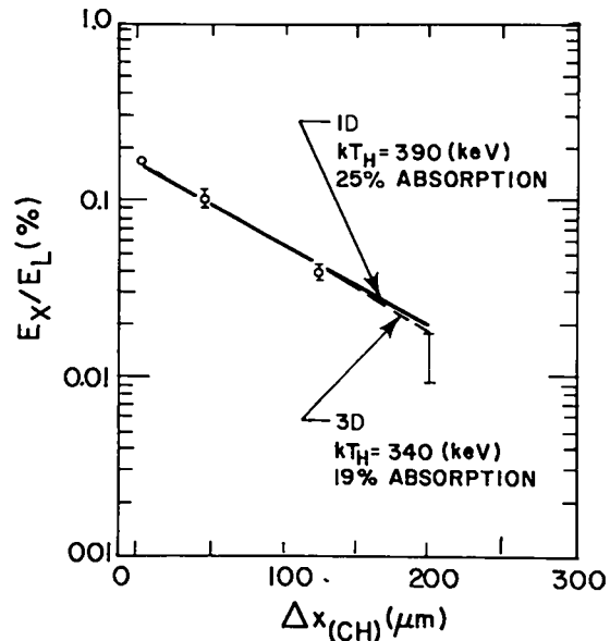
Fig. IV-10. Interpolated LASNEX suprathermal x-ray yield.
