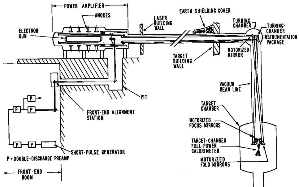
Fig. II-18. Beam-diagnostic location in the target-system beamline. The turning-chamber instrumentation package contains both calorimeter and temporal measuring devices.
