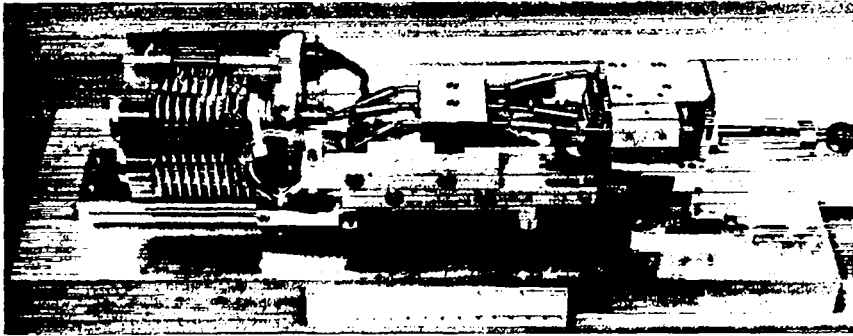
Fig. I-2. Electromechanical Hartmann target-alignment system.
