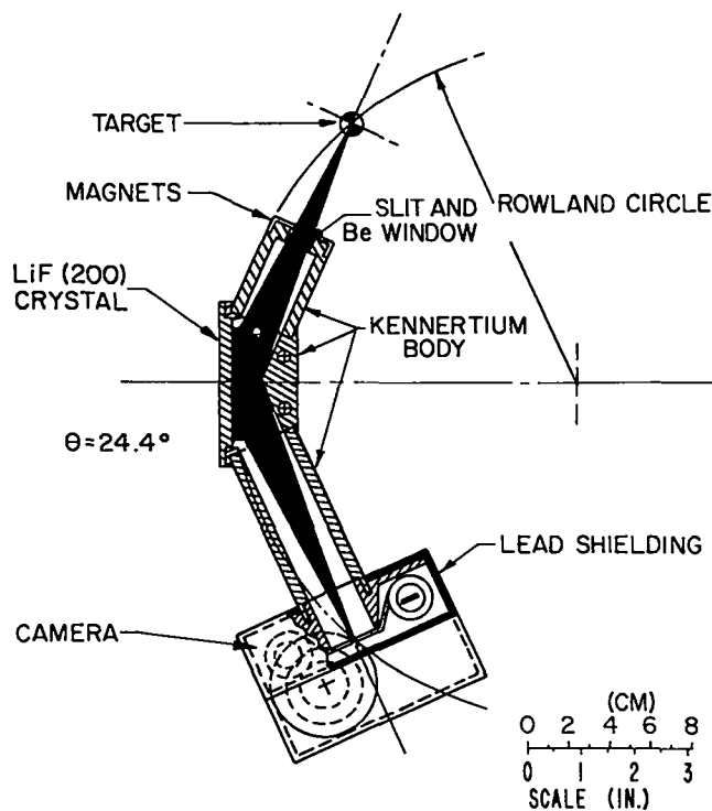
Fig. V-12. Curved-crystal spectrograph.
