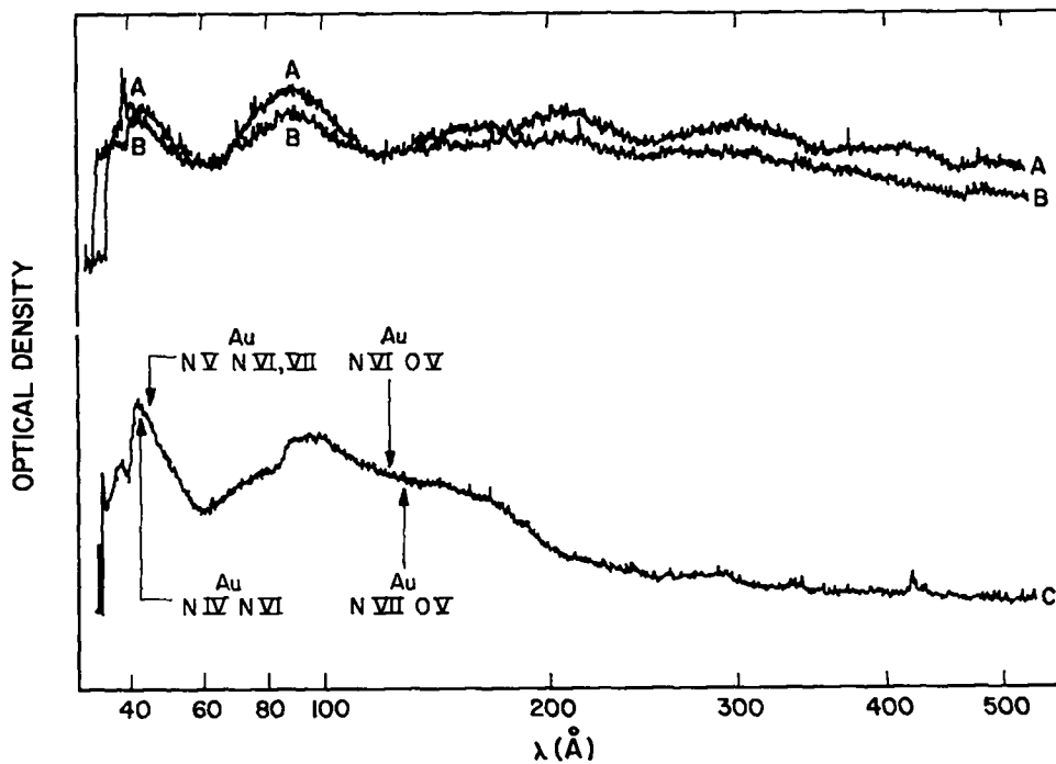
Fig. V-11. Microdensitometer scans of gold-coated GMBs: (a) 3- \mu\text{m} -thick gold coating, (b) 0.1- \mu\text{m} -thick gold coating of a 300- \mu\text{m} GMB plus 5- \mu\text{m} -thick CH, and (c) low-energy gold foil result at \sim 20 J. Laser energy in (a) and (b) was \sim 5 kJ.
