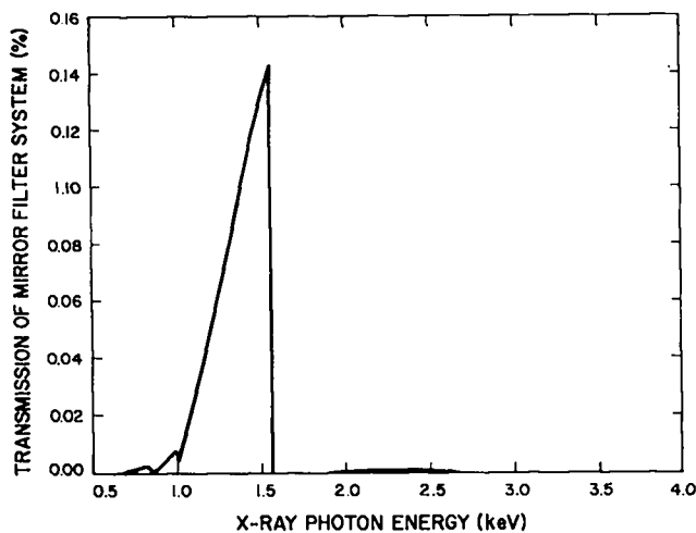
Fig. V-4. Spectral band pass of mirror collection system (with 10- \mu m aluminum foil filtration). Nickel mirror has 1.5 ^\circ grazing angle.
