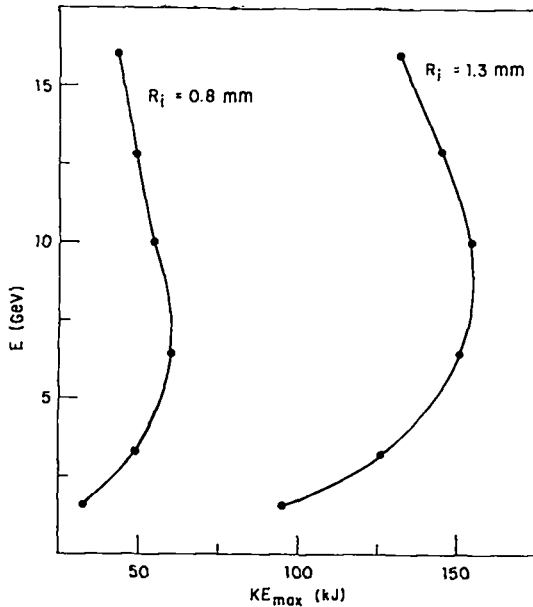
Fig. VIII-14. Ion particle energy vs maximum kinetic energy.
