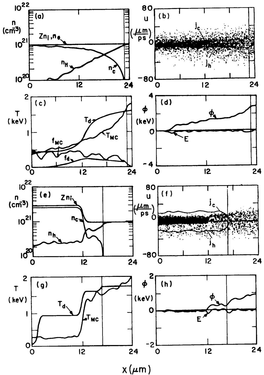
Fig. IV-6. An end-heated uniform plasma. (a)-(d). Transport through a density gradient. (e)-(h). j_{h,c} \approx 5 \times 10^{-21} n_{h,c} u_{h,c} ( u - \text{cm}^{-3}/\text{ps} ), E in arbitrary units.
