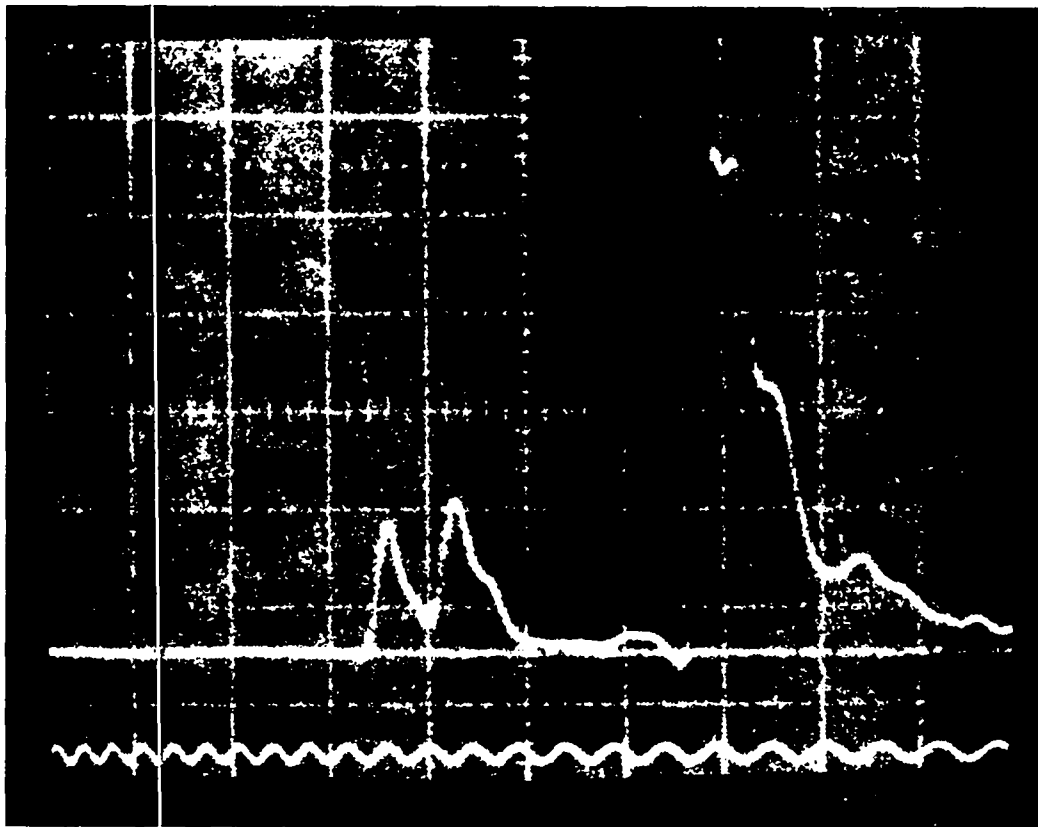
Fig. III-1. Temporally resolved backscatter from a 6.7- \mu\text{m} iron-coated spherical target. The two pulses at the left are identical samples of second-harmonic light Fresnel-reflected from the front and back surfaces of the salt window that provides the repulse signal. The single sample of 10.6- \mu\text{m} backscatter is optically delayed by 2.87 ns. Only one sample of 10.6- \mu\text{m} backscatter is obtained because one of the window surfaces is antireflection-coated for 10.6- \mu\text{m} light. The lower calibration trace is a 2-GHz sine wave.
